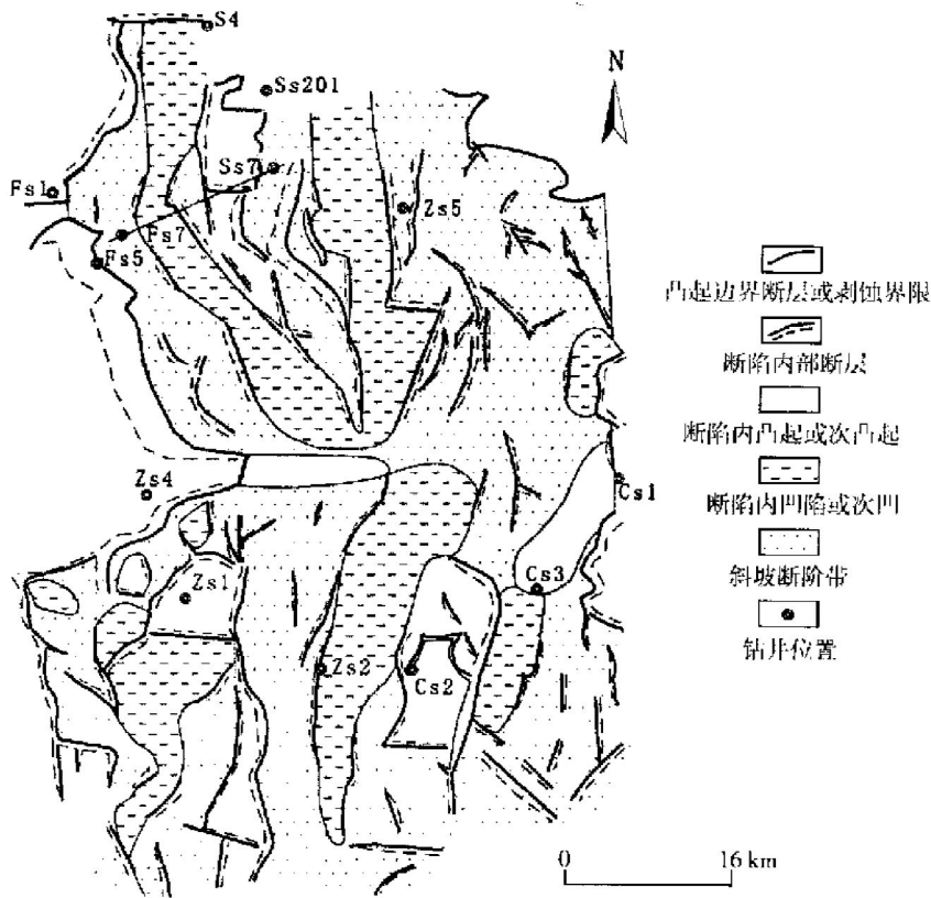
图 1 徐家围子断陷次级构造单元及断阶带的分布 Fig. 1 Distribution of secondary tectonic units and fault terrace belts in Xujiaweizi fault depression
